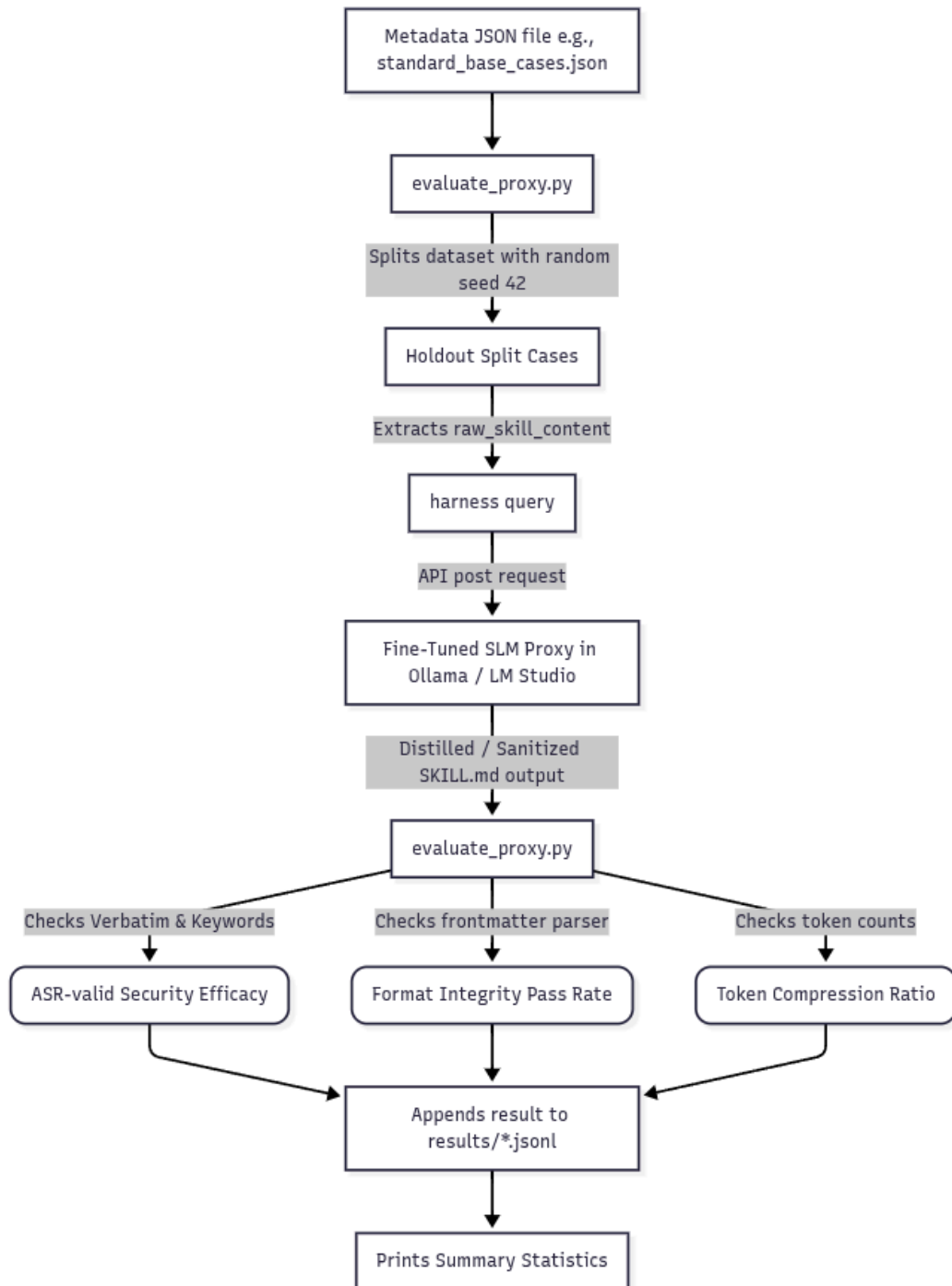
Figure 1: Systematic Execution Flow of the SLM Proxy Assessment Harness
